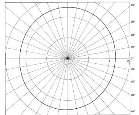
> AZIMUTH PATTERN (Typical azimuth patterns at 60° elevation) gain in dBi
